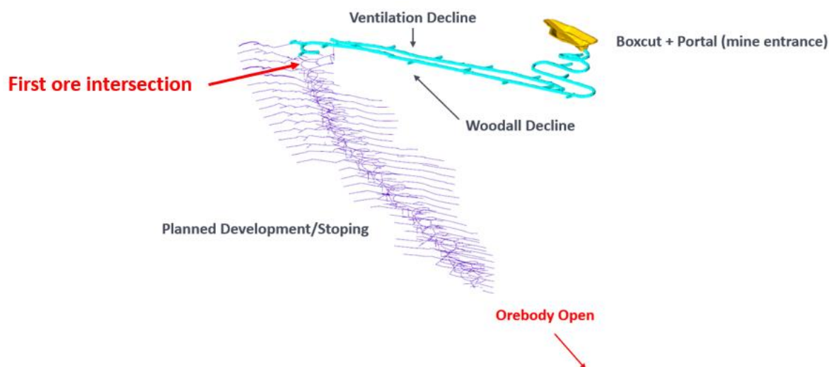
Figure 3 – Cassini Operation, location of First Ore (schematic)
